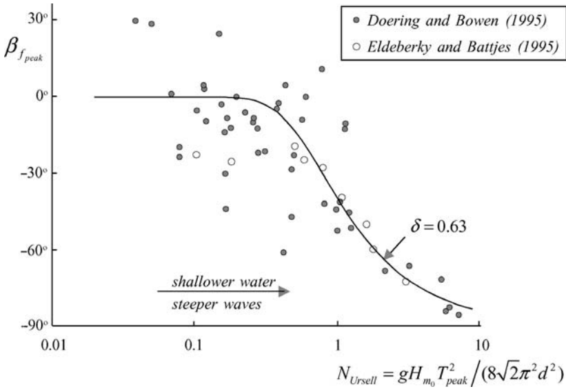
Figure 8.13 The observed evolution of the biphas of the self–self interaction at the peak frequency of a unimodal incident frequency spectrum as the waves enter shallow water (i.e., as a function of the Ursell number N_{Ursell} , see also Sections 5.6.1 and 9.3.3). The solid line represents Eq. (8.4.8) with \delta = 0.63 .
