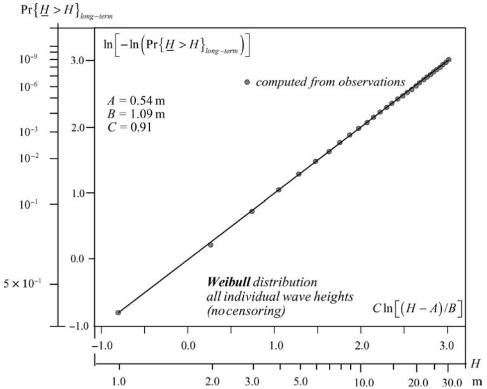
Figure 4.26 The long-term distribution of the individual wave height computed with the Battjes method, for the years 1980–2003 for NODC buoy 46005 of Figs. 4.17 and 4.18 (not censored) and plotted with Weibull scales. The straight line represents the best-fit candidate distribution (least-squares). The value of the shape parameter C = 0.91 , reduces this Weibull distribution to nearly an exponential distribution (for which C = 1 ).
