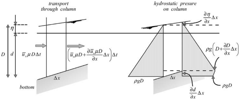
Figure E.1 A property \mu being transported by the water in the x -direction through a column, and the hydrostatic pressure on that column.
