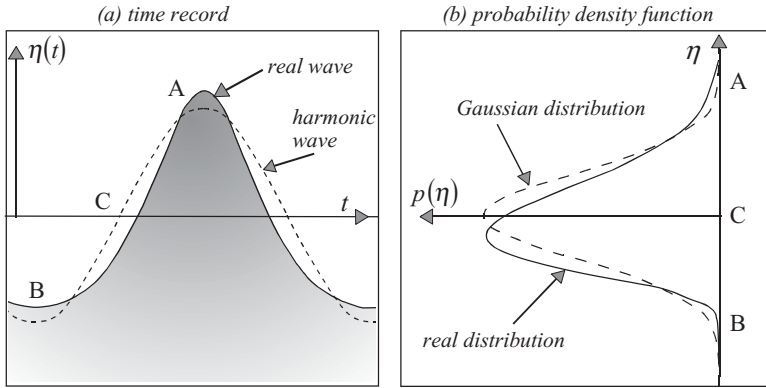
Figure 4.2 The analogy of the difference between a harmonic wave and a real (Stokes-type) wave (panel a) and the corresponding difference between a Gaussian distribution and the real (observed) probability density function of the surface elevation \eta at sea (panel b). Note that the axes in panel (b) are rotated 90^\circ counter-clockwise relative to the usual orientation (to show \eta vertically, as in panel a).
