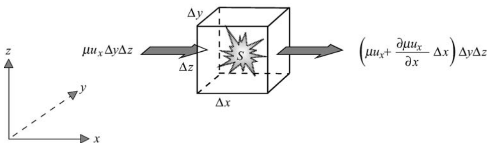
Figure 5.1 A property \mu being transported by the water in the x -direction, through a volume \Delta x \Delta y \Delta z in a three-dimensional situation.
